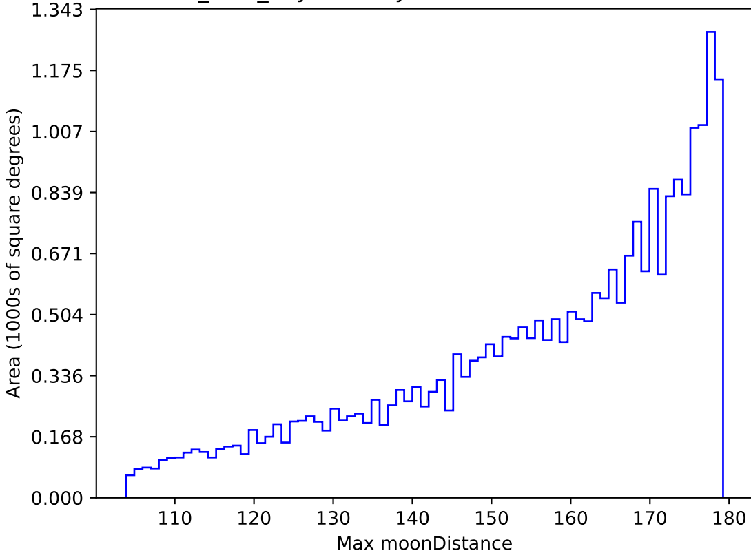
noroll_v3.4_10yrs All sky r band: Max moonDistance
