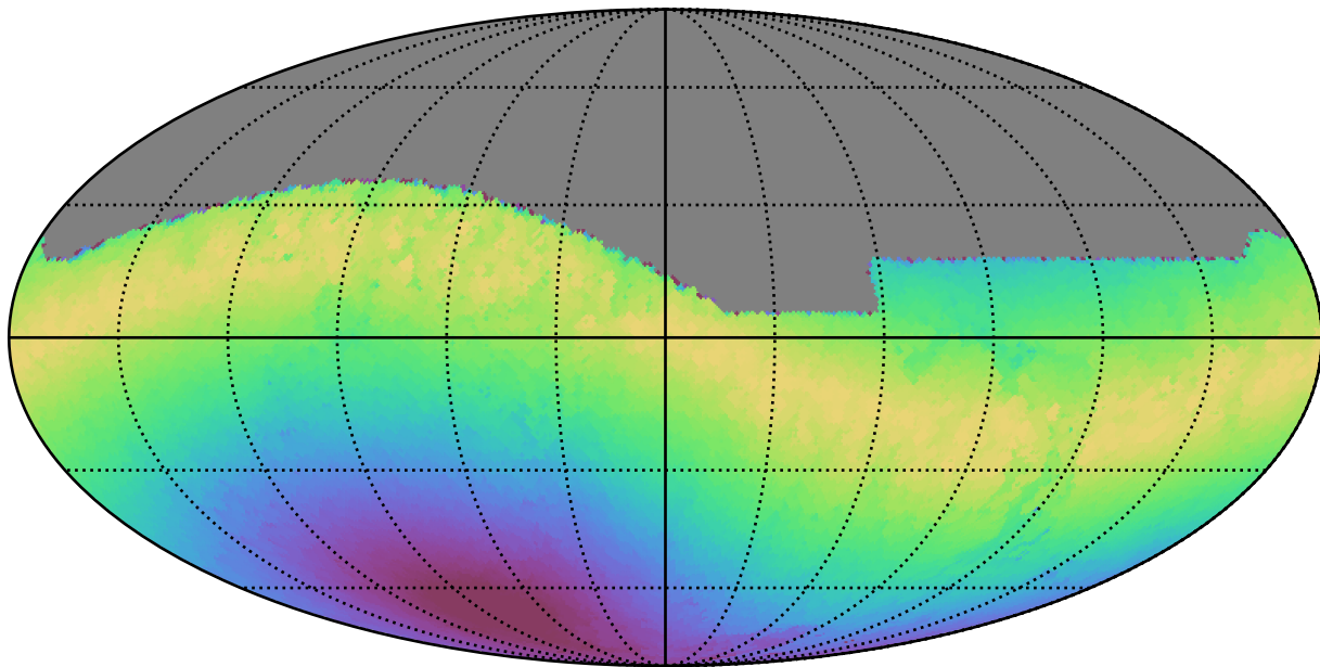
noroll_v3.4_10yrs All sky i band: Max moonDistance
