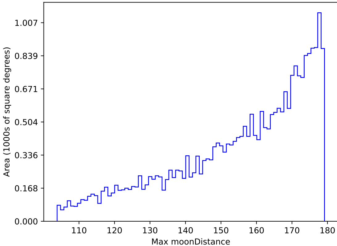
noroll_v3.4_10yrs All sky i band: Max moonDistance
