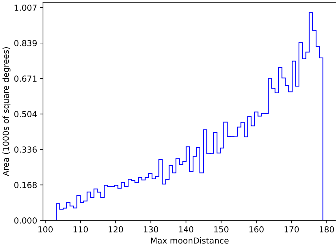
noroll_v3.4_10yrs All sky g band: Max moonDistance
