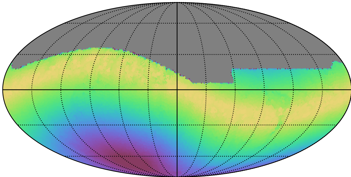
noroll_v3.4_10yrs All sky all bands: Max moonDistance
