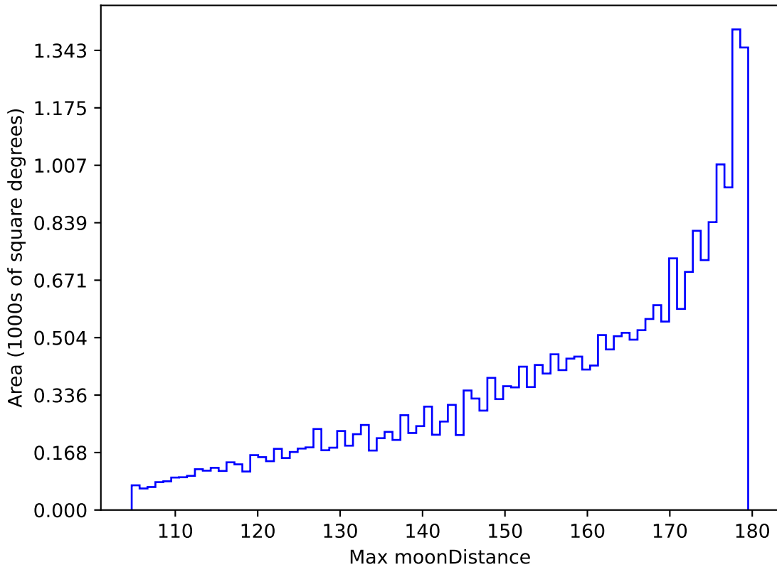
noroll_v3.4_10yrs All sky all bands: Max moonDistance
