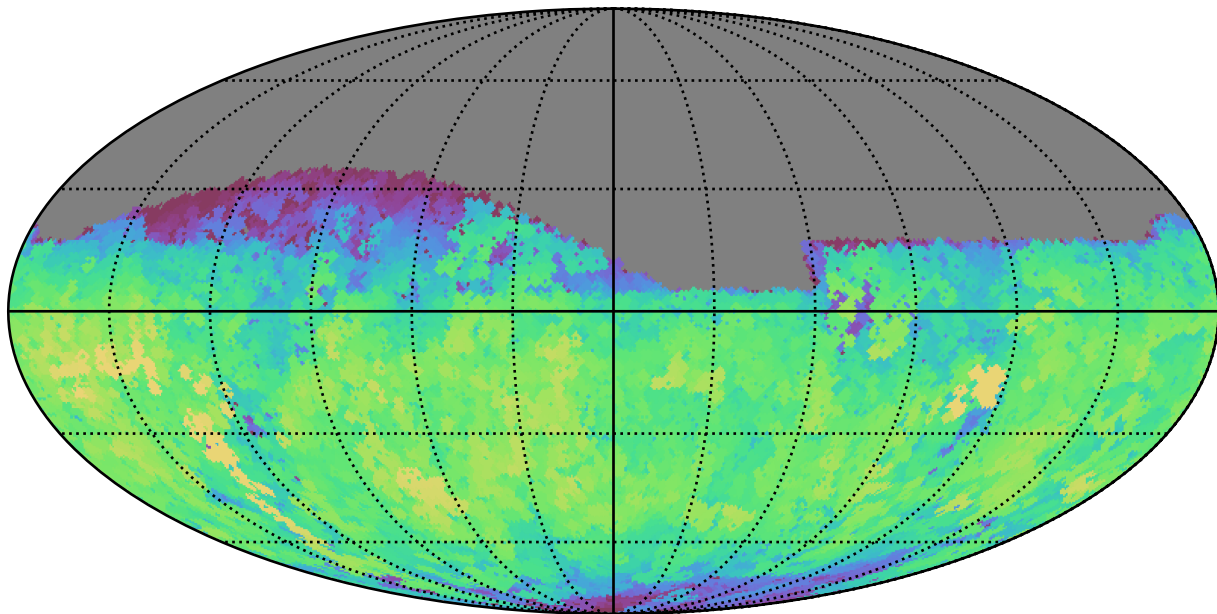
noroll_v3.4_10yrs Yr 1 z band: Max fiveSigmaDepth
