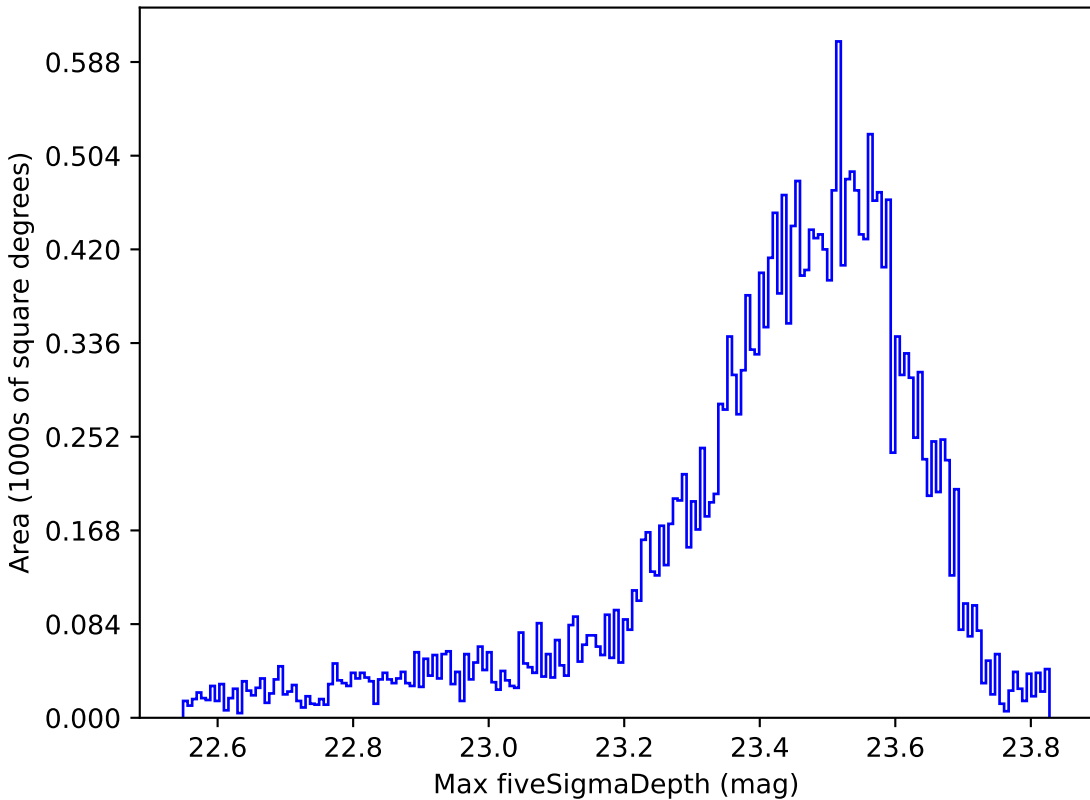
noroll_v3.4_10yrs Yr 1 z band: Max fiveSigmaDepth
