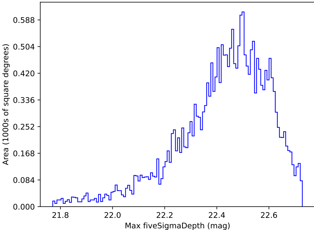
noroll_v3.4_10yrs Yr 1 y band: Max fiveSigmaDepth
