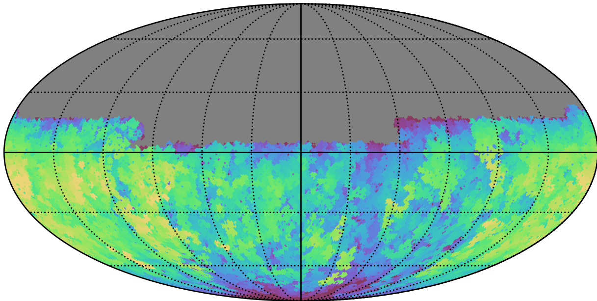
noroll_v3.4_10yrs Yr 1 u band: Max fiveSigmaDepth
