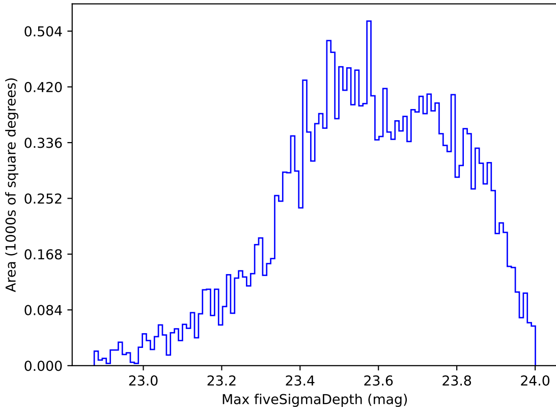
noroll_v3.4_10yrs Yr 1 u band: Max fiveSigmaDepth
