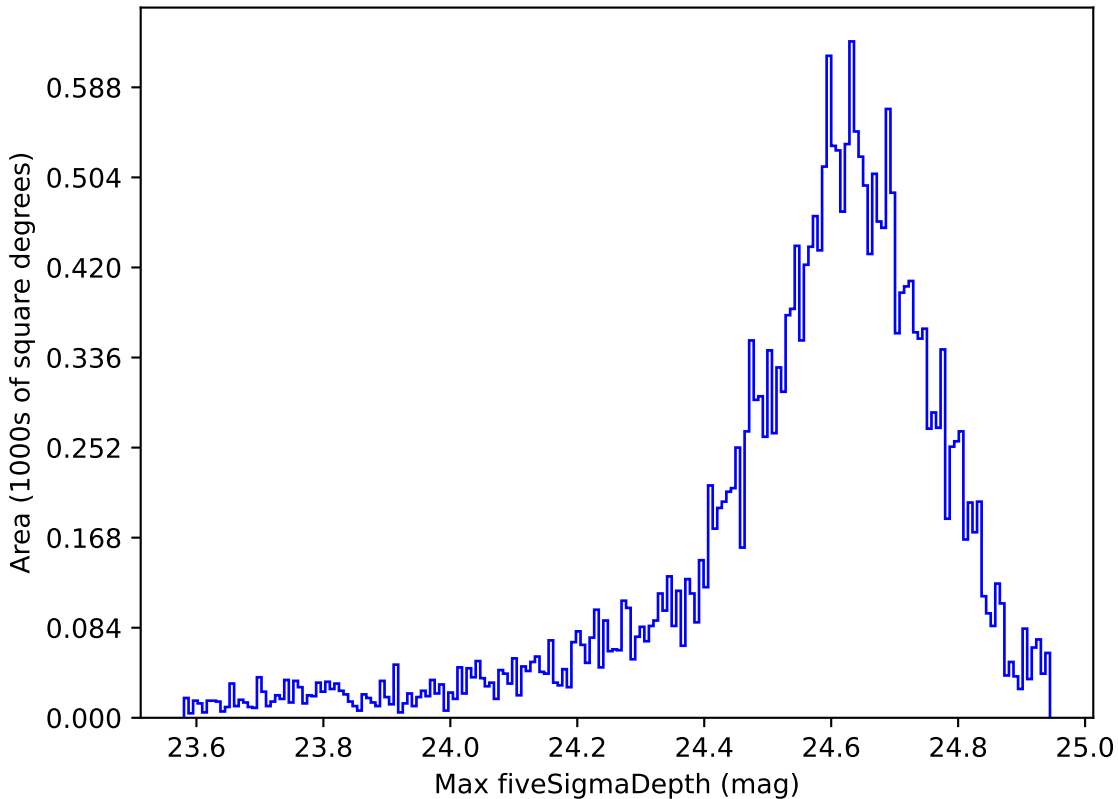
noroll_v3.4_10yrs Yr 1 r band: Max fiveSigmaDepth
