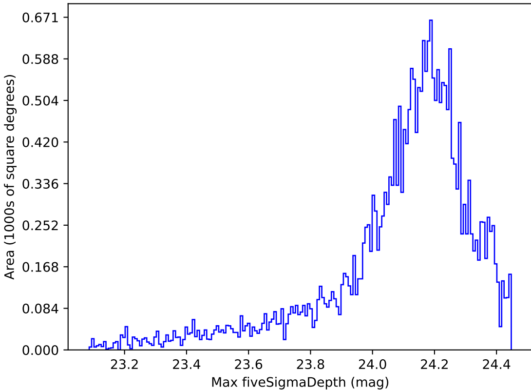
noroll_v3.4_10yrs Yr 1 i band: Max fiveSigmaDepth
