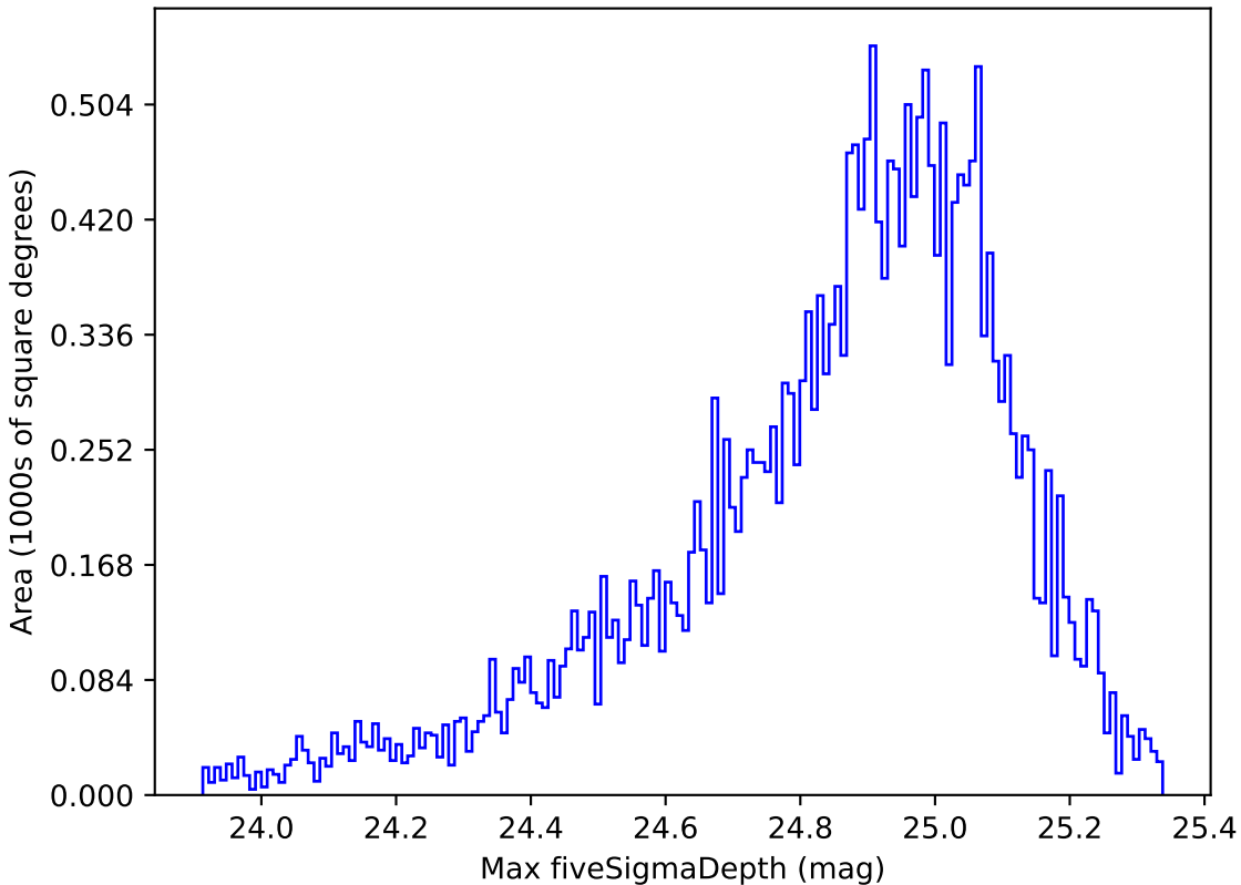
noroll_v3.4_10yrs Yr 1 g band: Max fiveSigmaDepth
