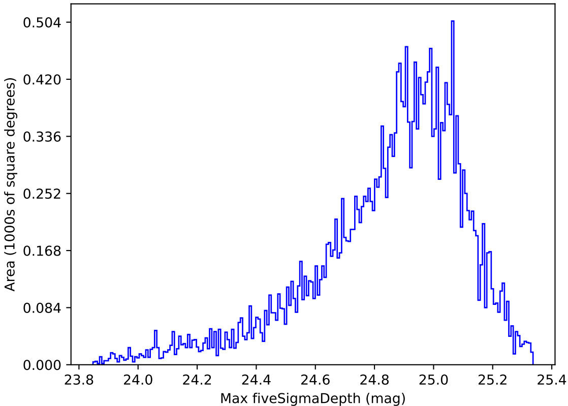
noroll_v3.4_10yrs Yr 1 all bands: Max fiveSigmaDepth
