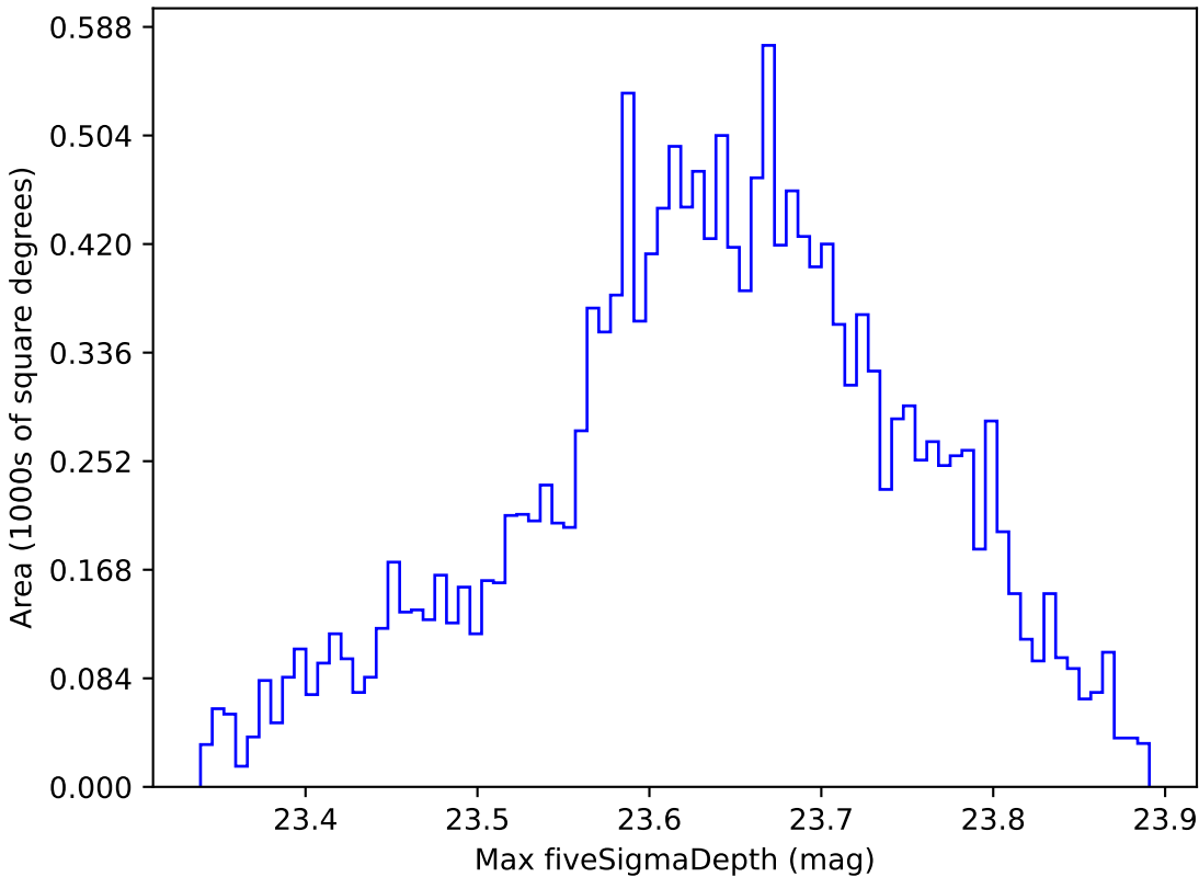
noroll_v3.4_10yrs WFD z band: Max fiveSigmaDepth
