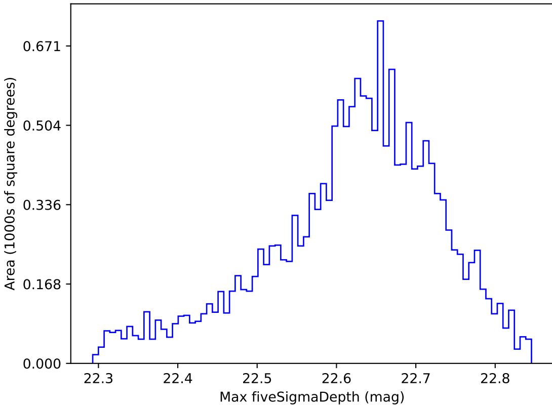
noroll_v3.4_10yrs WFD y band: Max fiveSigmaDepth
