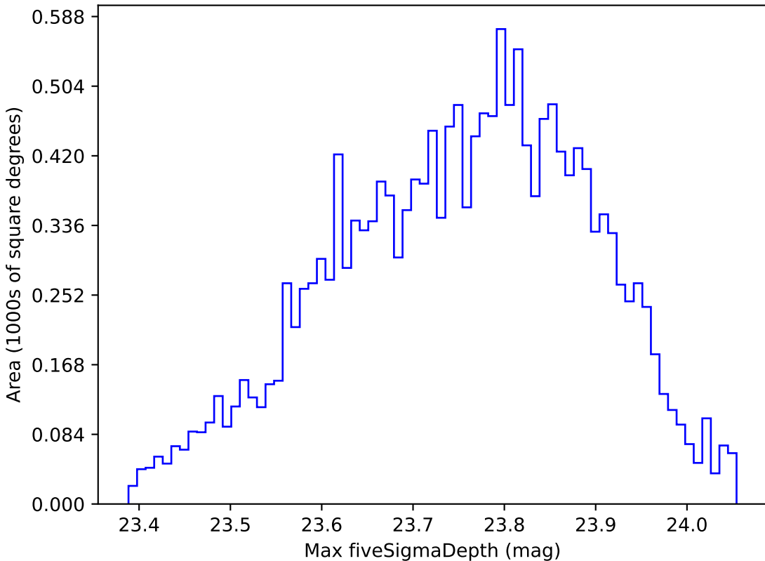
noroll_v3.4_10yrs WFD u band: Max fiveSigmaDepth
