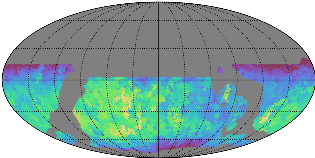
noroll_v3.4_10yrs WFD r band: Max fiveSigmaDepth
