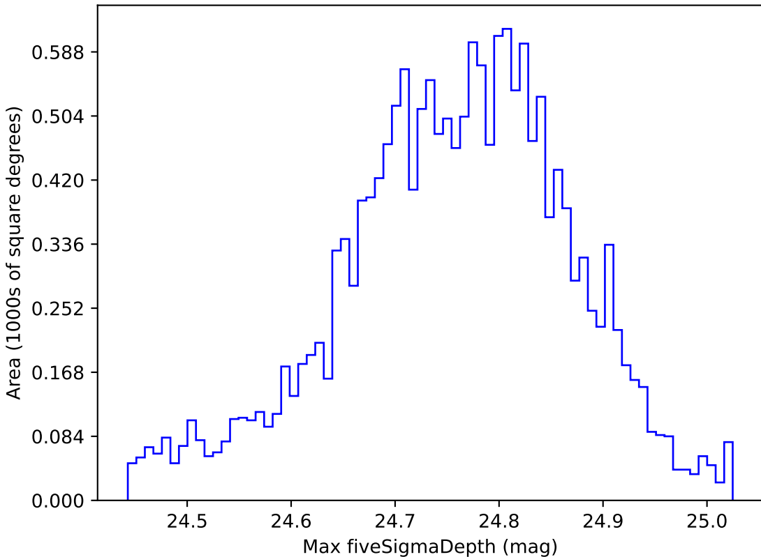
noroll_v3.4_10yrs WFD r band: Max fiveSigmaDepth
