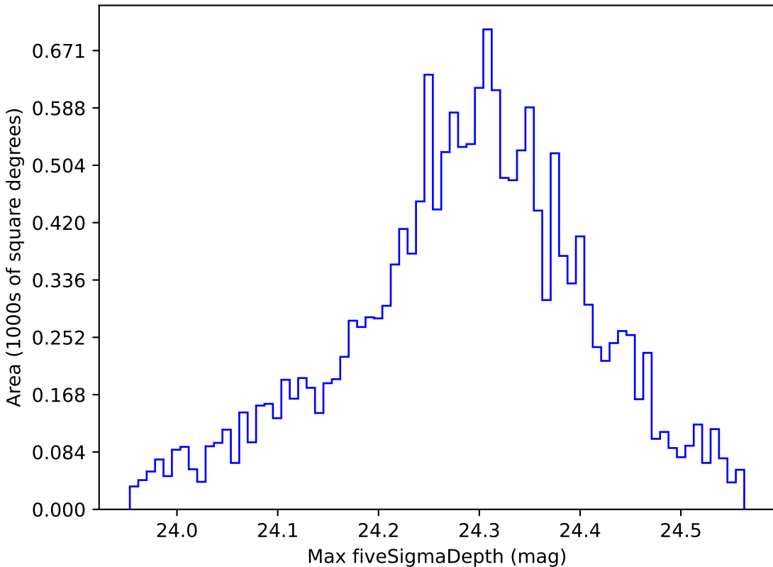
noroll_v3.4_10yrs WFD i band: Max fiveSigmaDepth
