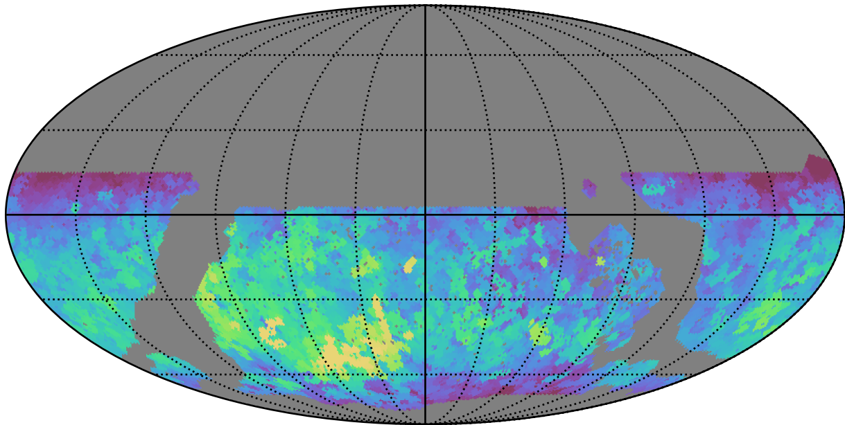
noroll_v3.4_10yrs WFD g band: Max fiveSigmaDepth
