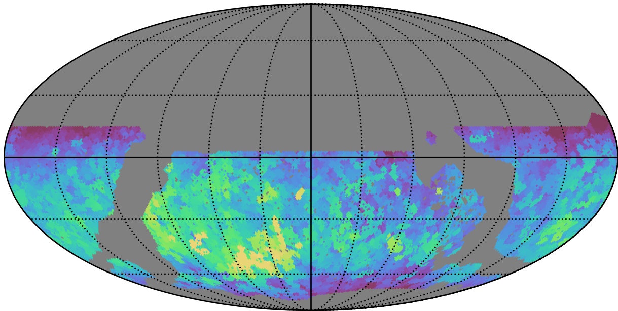
noroll_v3.4_10yrs WFD all bands: Max fiveSigmaDepth
