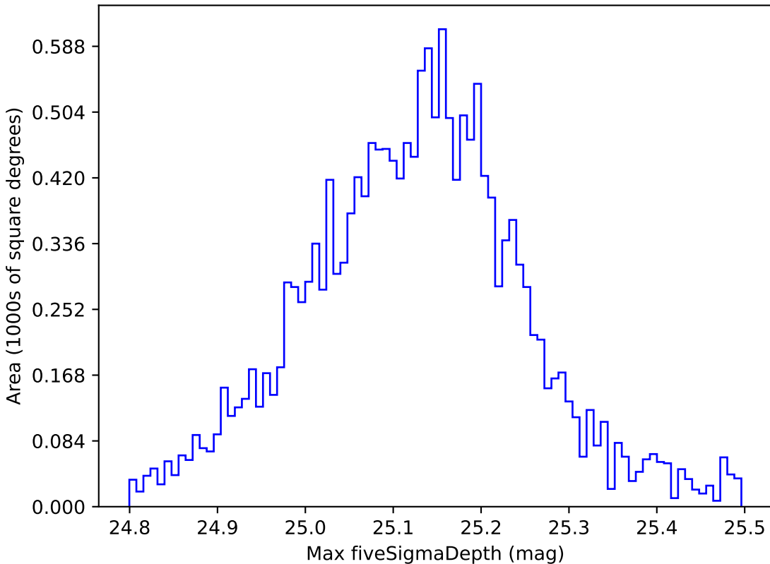
noroll_v3.4_10yrs WFD all bands: Max fiveSigmaDepth
