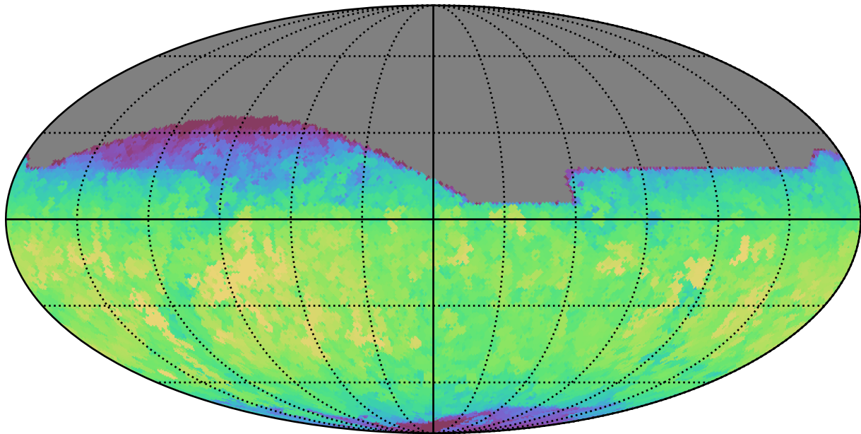
noroll_v3.4_10yrs All sky z band: Max fiveSigmaDepth
