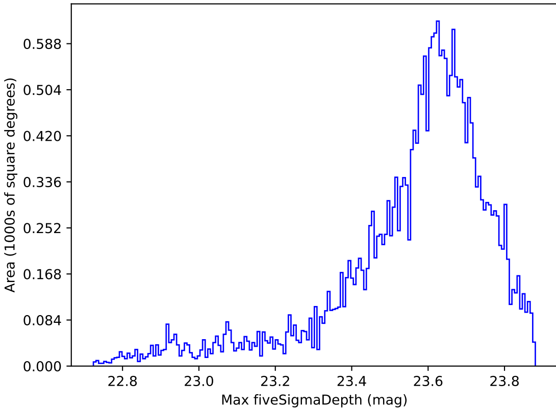
noroll_v3.4_10yrs All sky z band: Max fiveSigmaDepth
