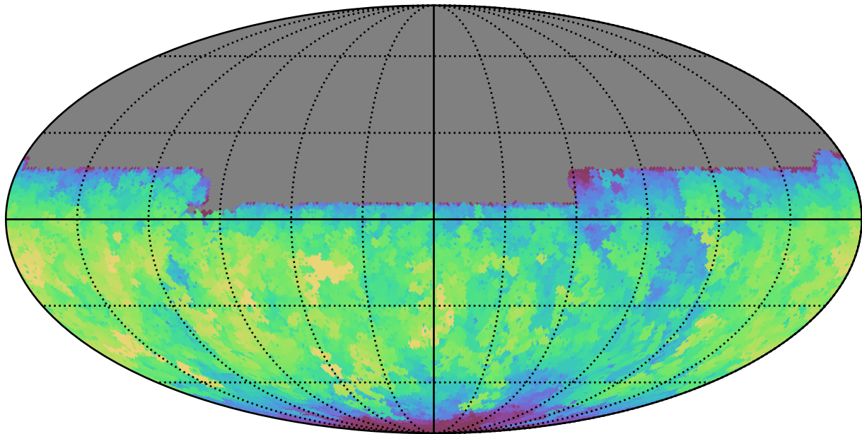
noroll_v3.4_10yrs All sky u band: Max fiveSigmaDepth
