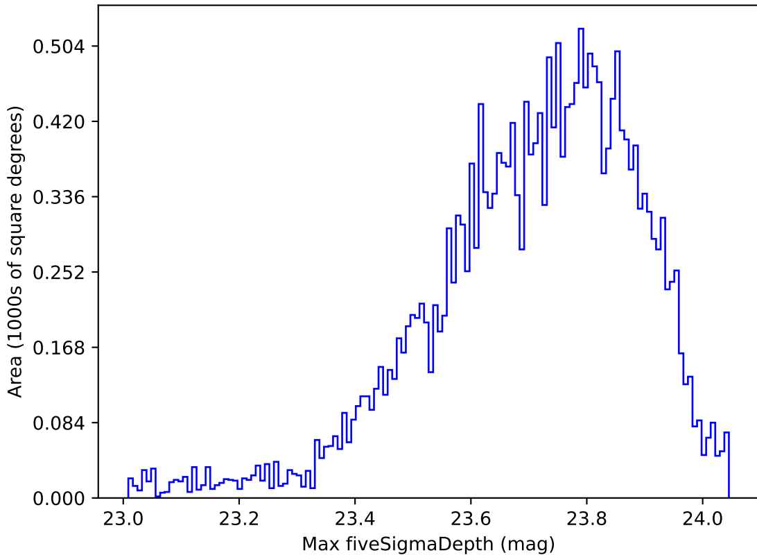
noroll_v3.4_10yrs All sky u band: Max fiveSigmaDepth
