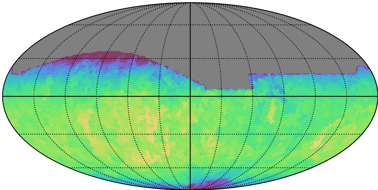
noroll_v3.4_10yrs All sky r band: Max fiveSigmaDepth
