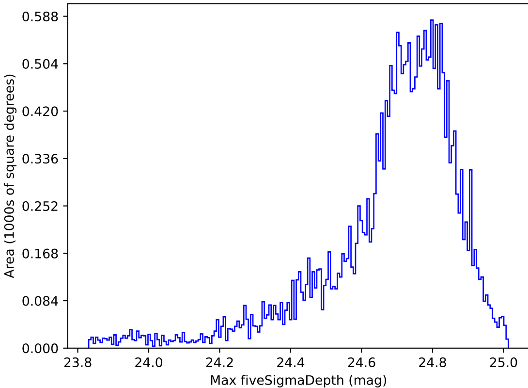
noroll_v3.4_10yrs All sky r band: Max fiveSigmaDepth
