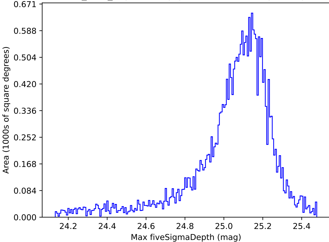
noroll_v3.4_10yrs All sky g band: Max fiveSigmaDepth
