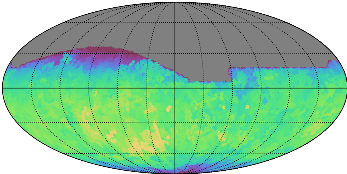
noroll_v3.4_10yrs All sky all bands: Max fiveSigmaDepth
