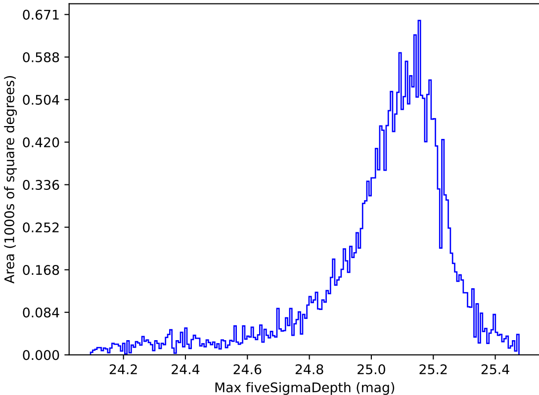
noroll_v3.4_10yrs All sky all bands: Max fiveSigmaDepth
