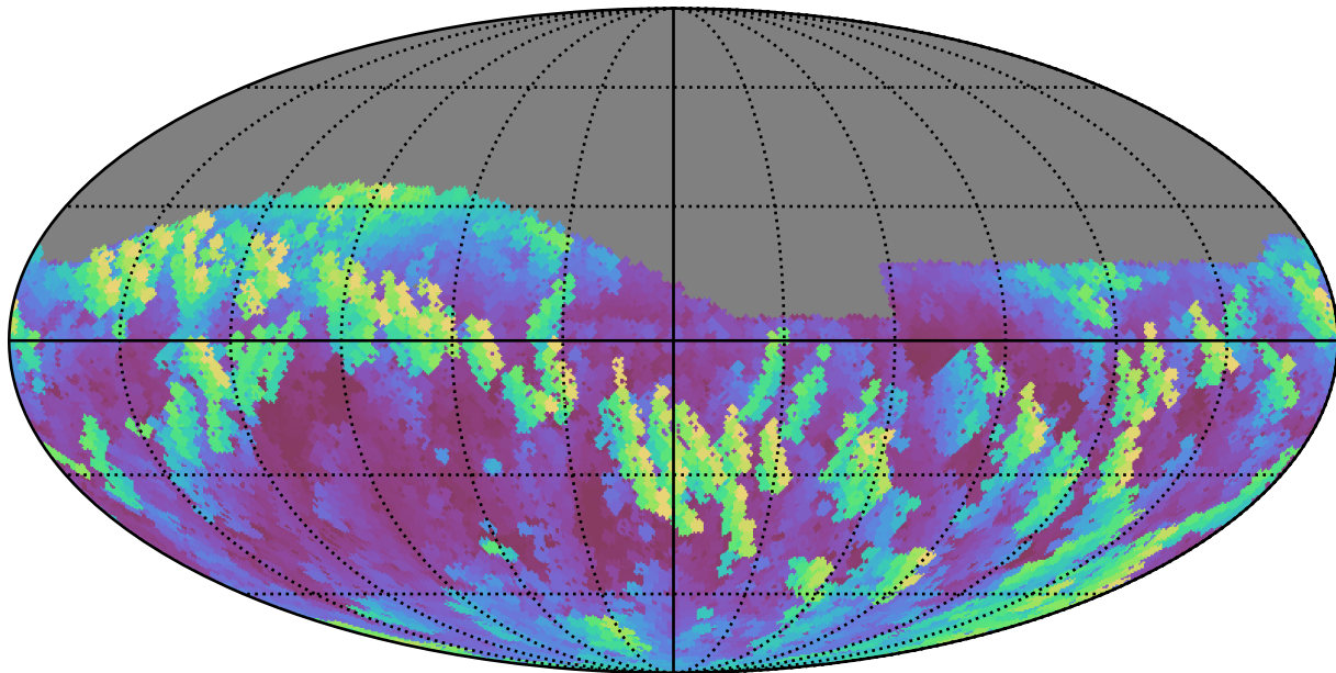
noroll_v3.4_10yrs Yr 1 z band: Max airmass
