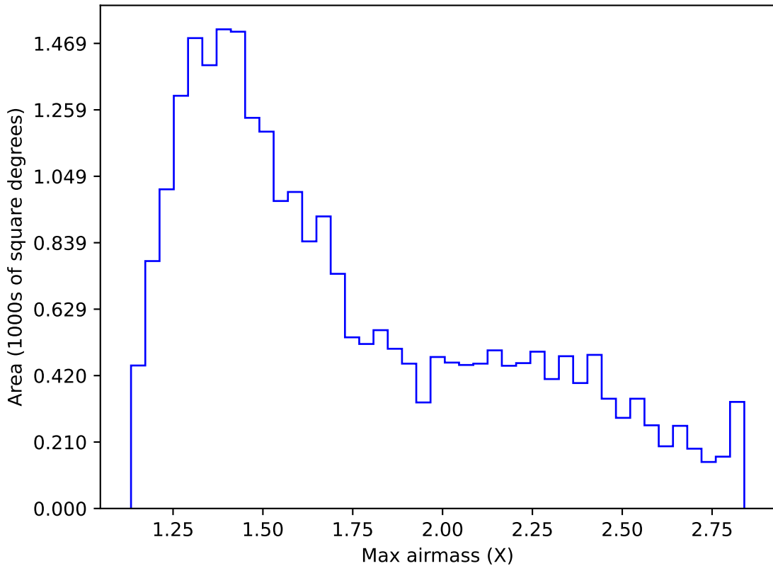
noroll_v3.4_10yrs Yr 1 z band: Max airmass
