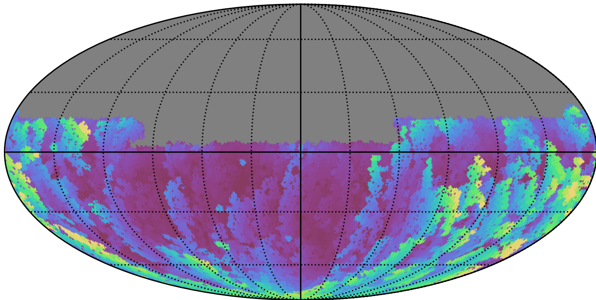
noroll_v3.4_10yrs Yr 1 u band: Max airmass
