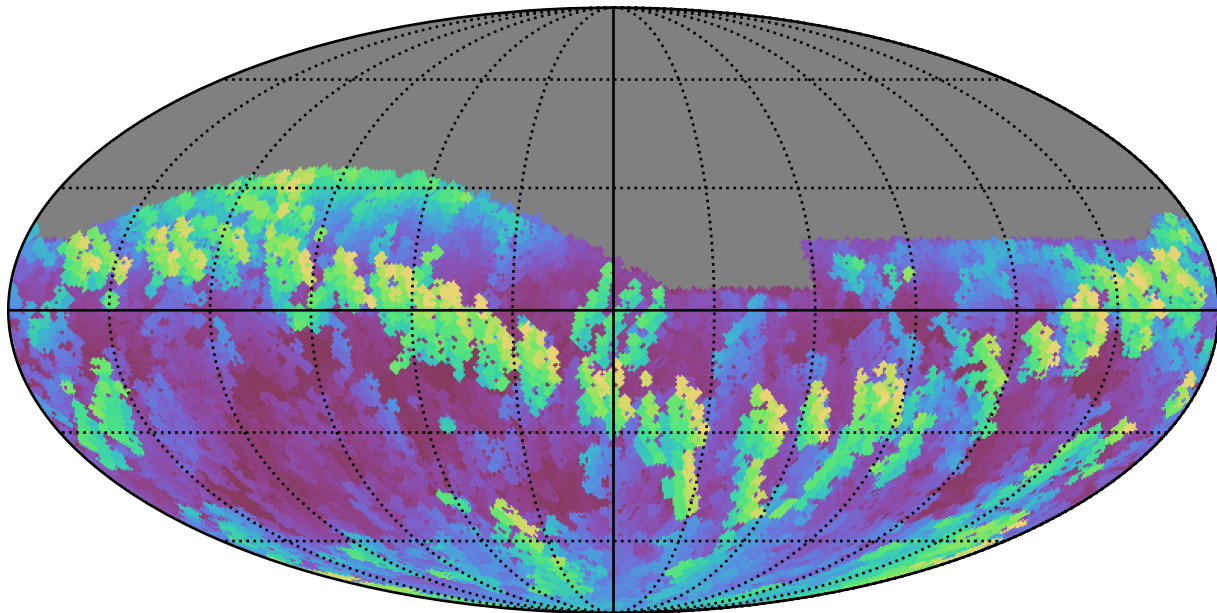
noroll_v3.4_10yrs Yr 1 i band: Max airmass
