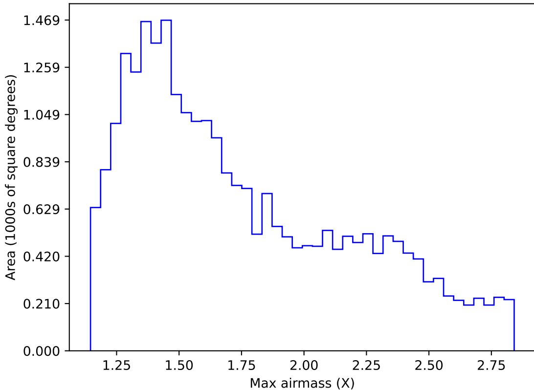
noroll_v3.4_10yrs Yr 1 i band: Max airmass
