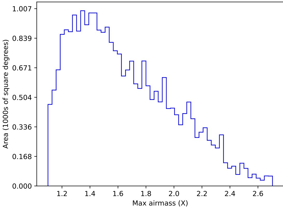
noroll_v3.4_10yrs Yr 1 g band: Max airmass
