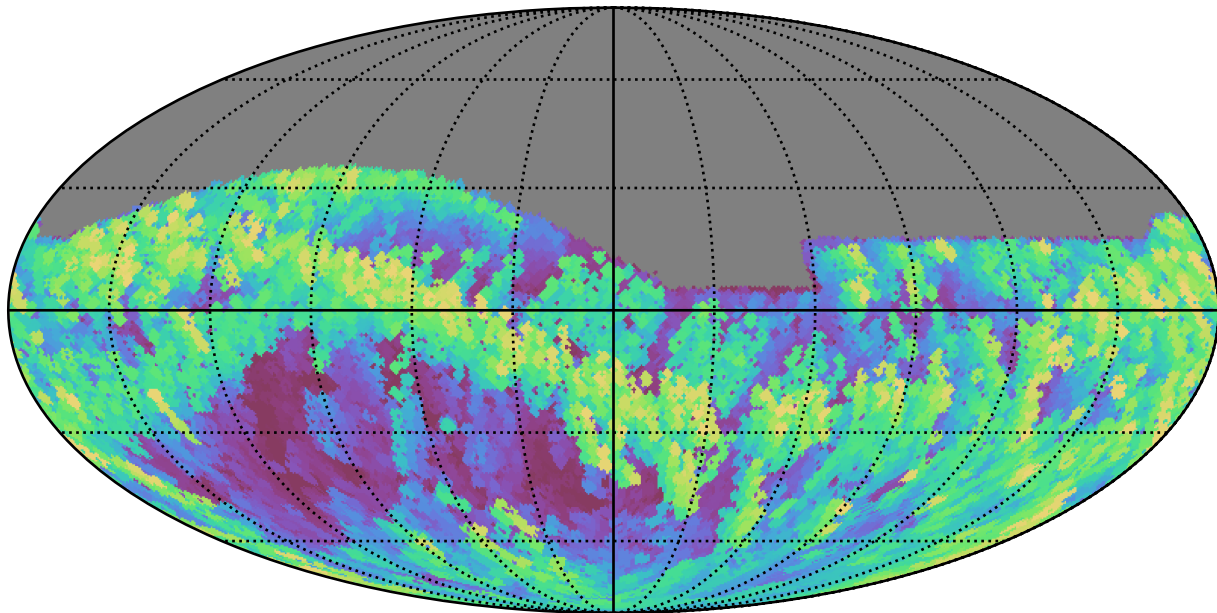
noroll_v3.4_10yrs Yr 1 all bands: Max airmass
