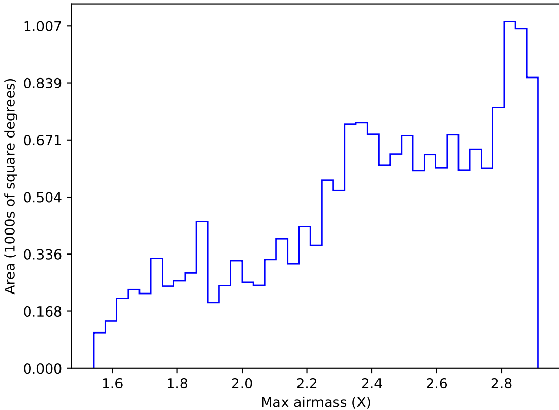
noroll_v3.4_10yrs WFD z band: Max airmass
