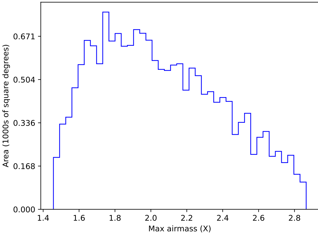
noroll_v3.4_10yrs WFD y band: Max airmass
