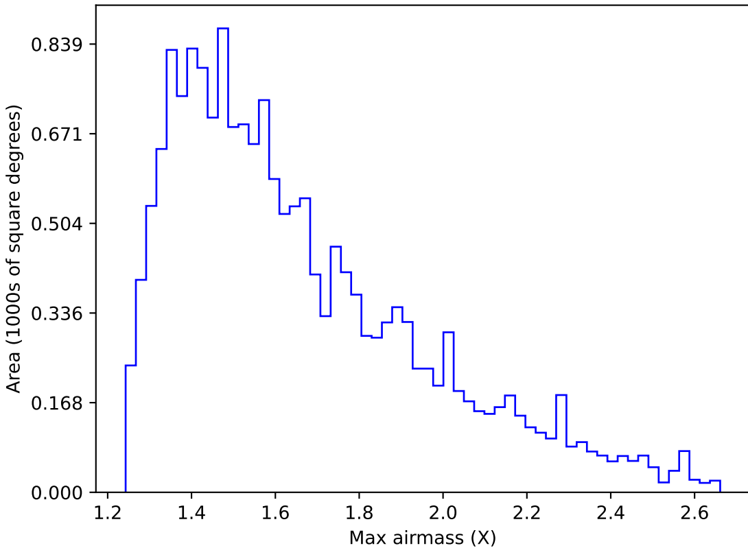
noroll_v3.4_10yrs WFD u band: Max airmass
