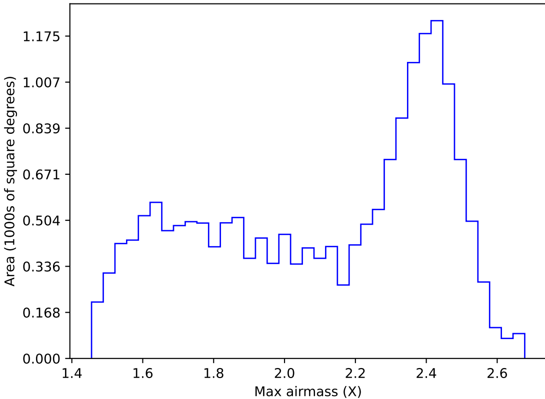
noroll_v3.4_10yrs WFD r band: Max airmass
