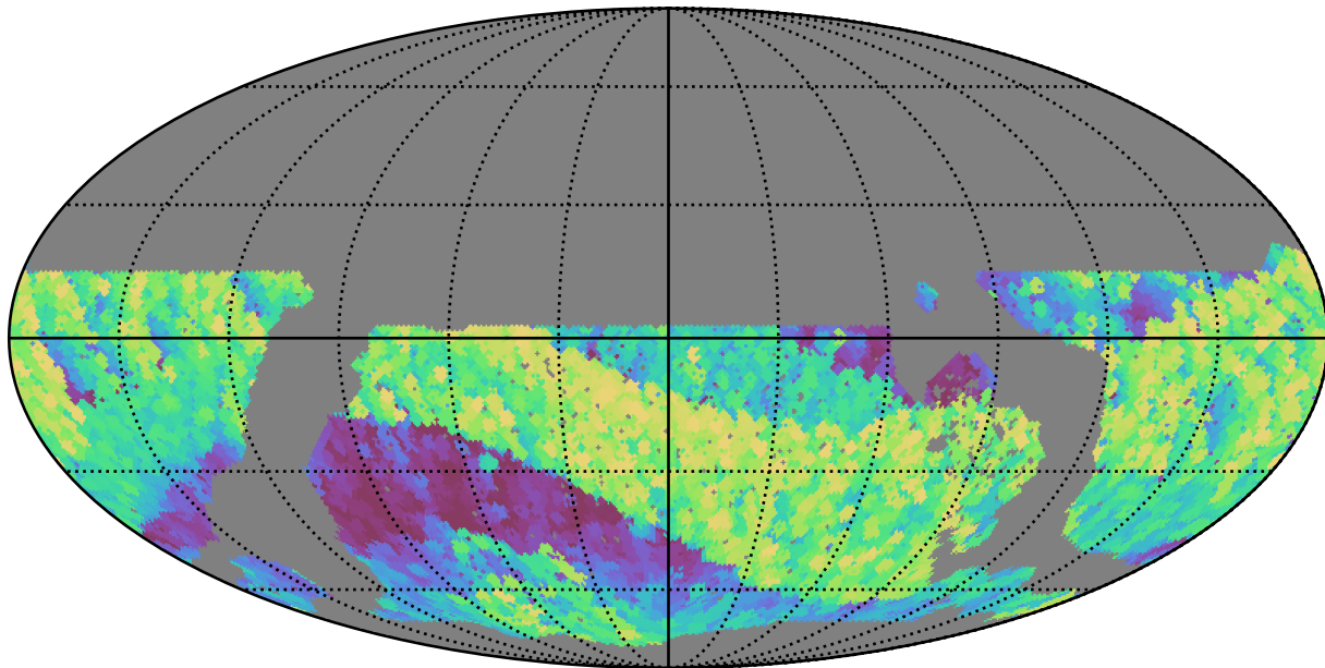
noroll_v3.4_10yrs WFD i band: Max airmass
