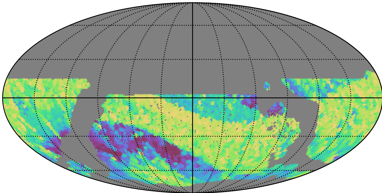
noroll_v3.4_10yrs WFD all bands: Max airmass
