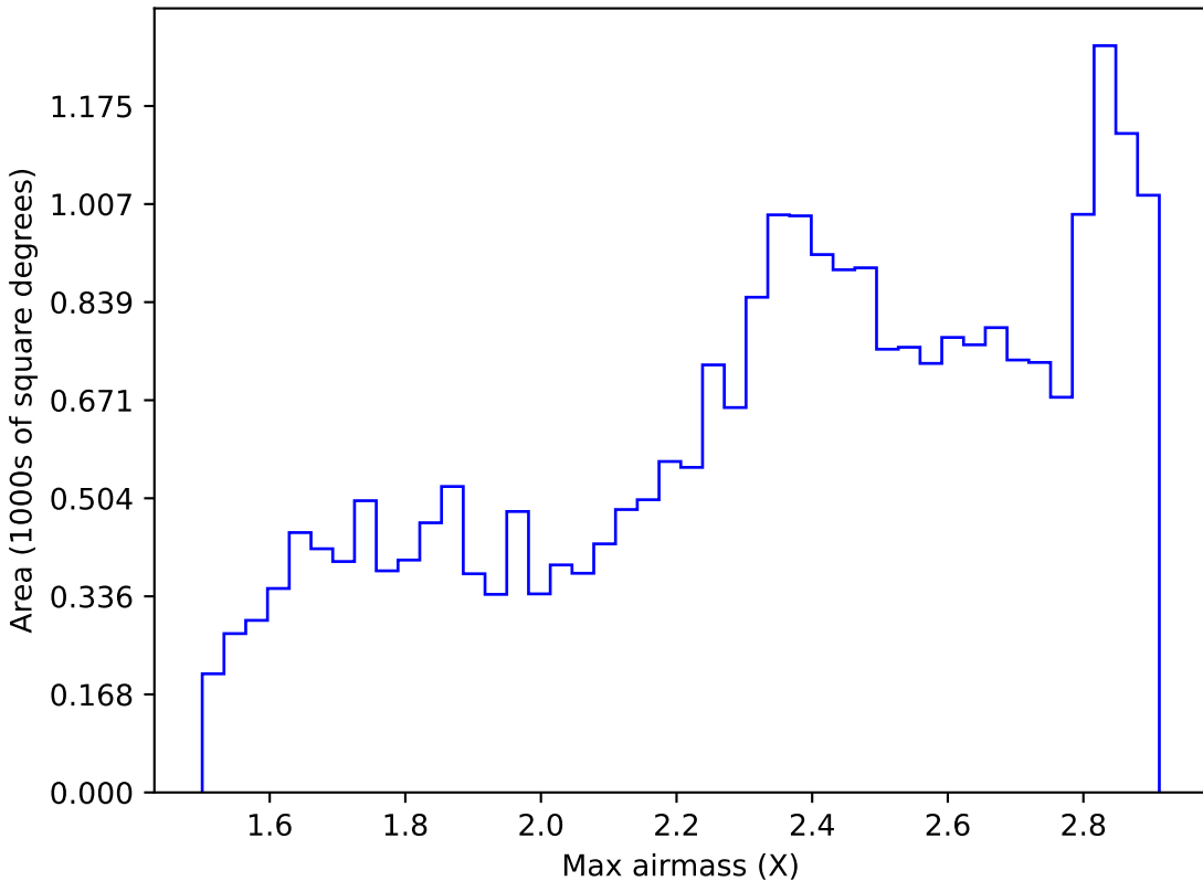
noroll_v3.4_10yrs All sky z band: Max airmass
