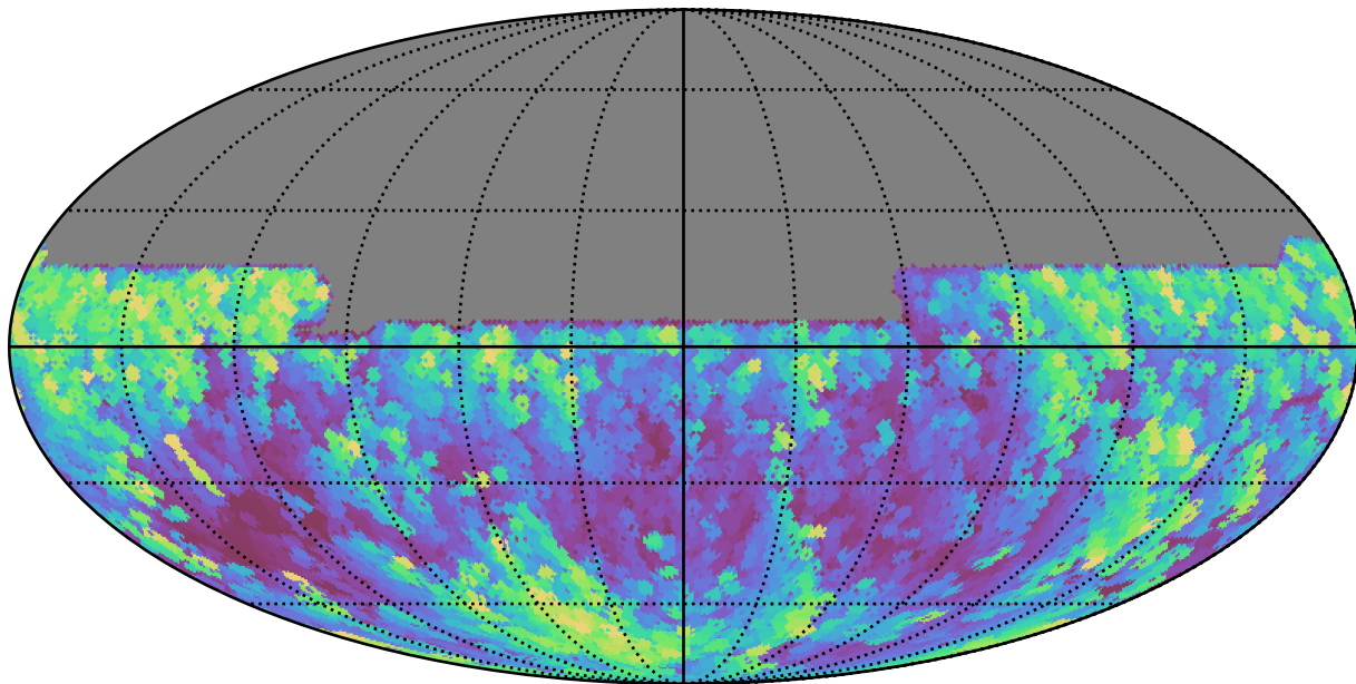
noroll_v3.4_10yrs All sky y band: Max airmass
