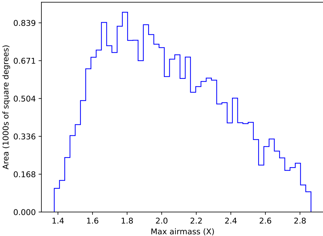
noroll_v3.4_10yrs All sky y band: Max airmass
