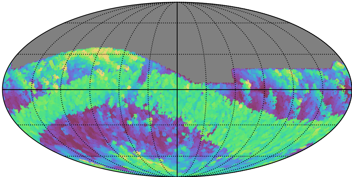
noroll_v3.4_10yrs All sky r band: Max airmass
